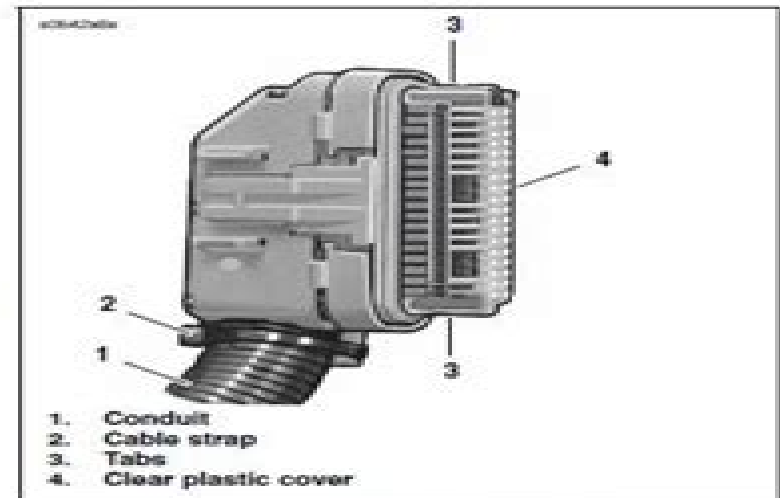
Figure 6-30. ECM Connector
