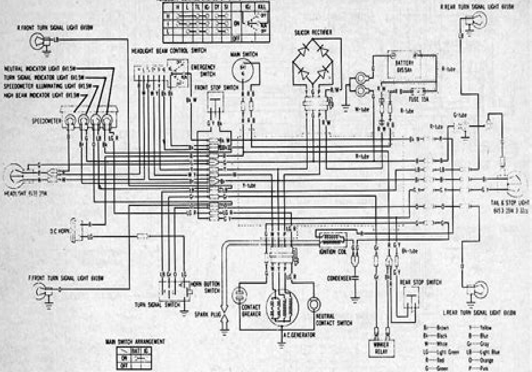
HEADLIGHT CONTROL (EMERGENCY SWITCH ARRANGEMENT)
