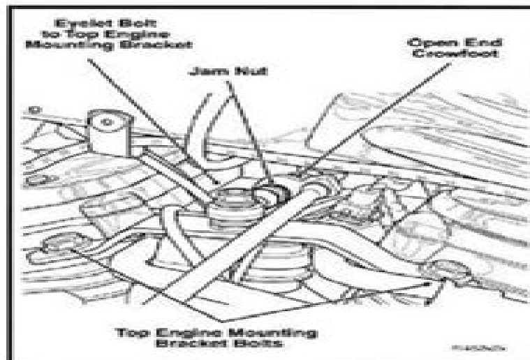
Figure 1-22. Top Stabilizer Link and Engine Mounting Bracket Bolts (Left Side View)
