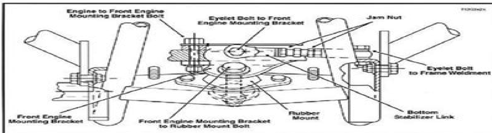
Figure 1-23. Bottom Stabilizer Link and Front Engine Mount Bolts
