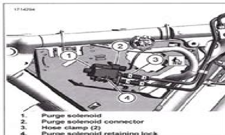
Figure 6-37. Purge Solenoid (behind left side caddy)
