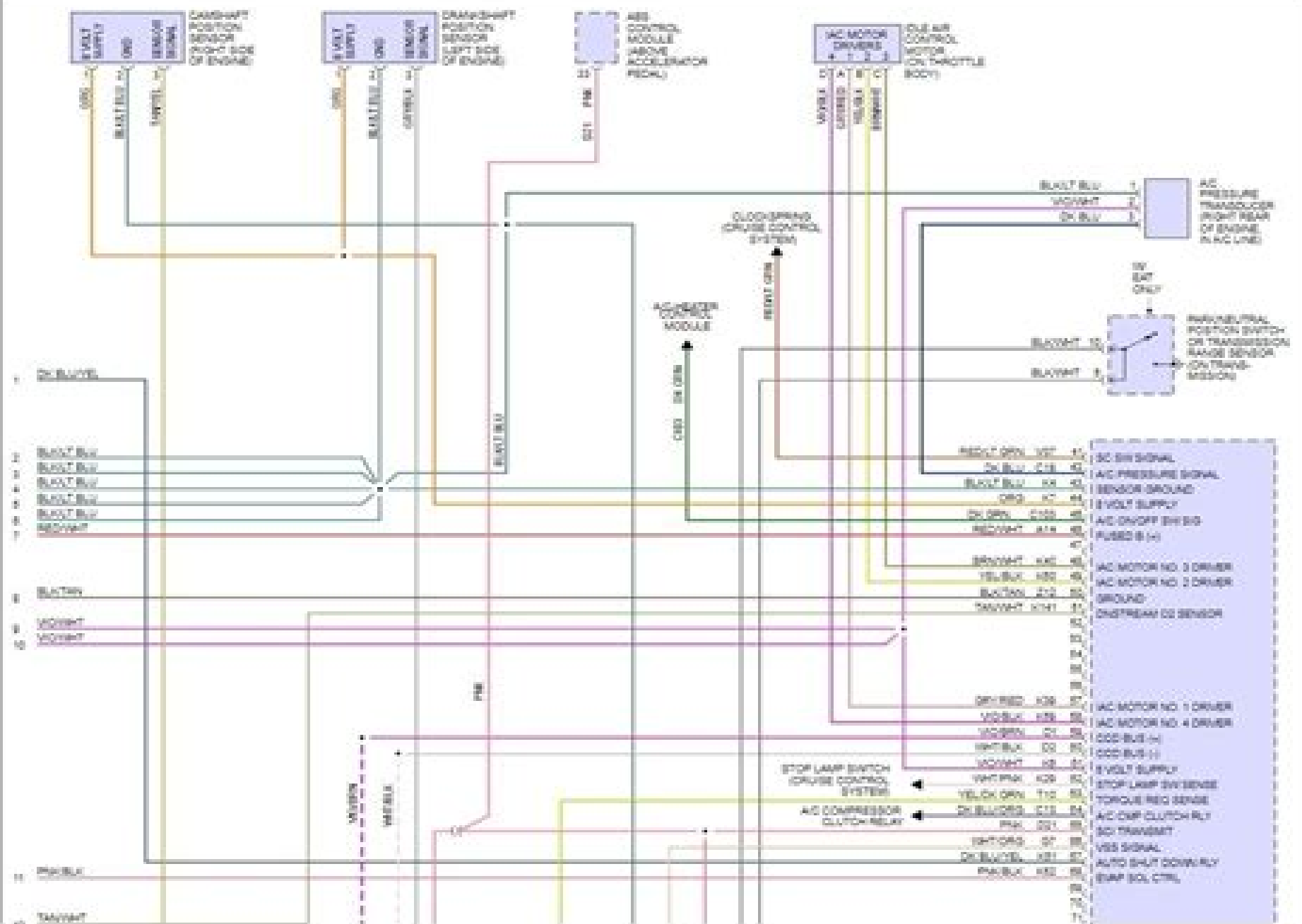
Fig 6: 3.3L, Engine Performance Circuits (3 of 3)
