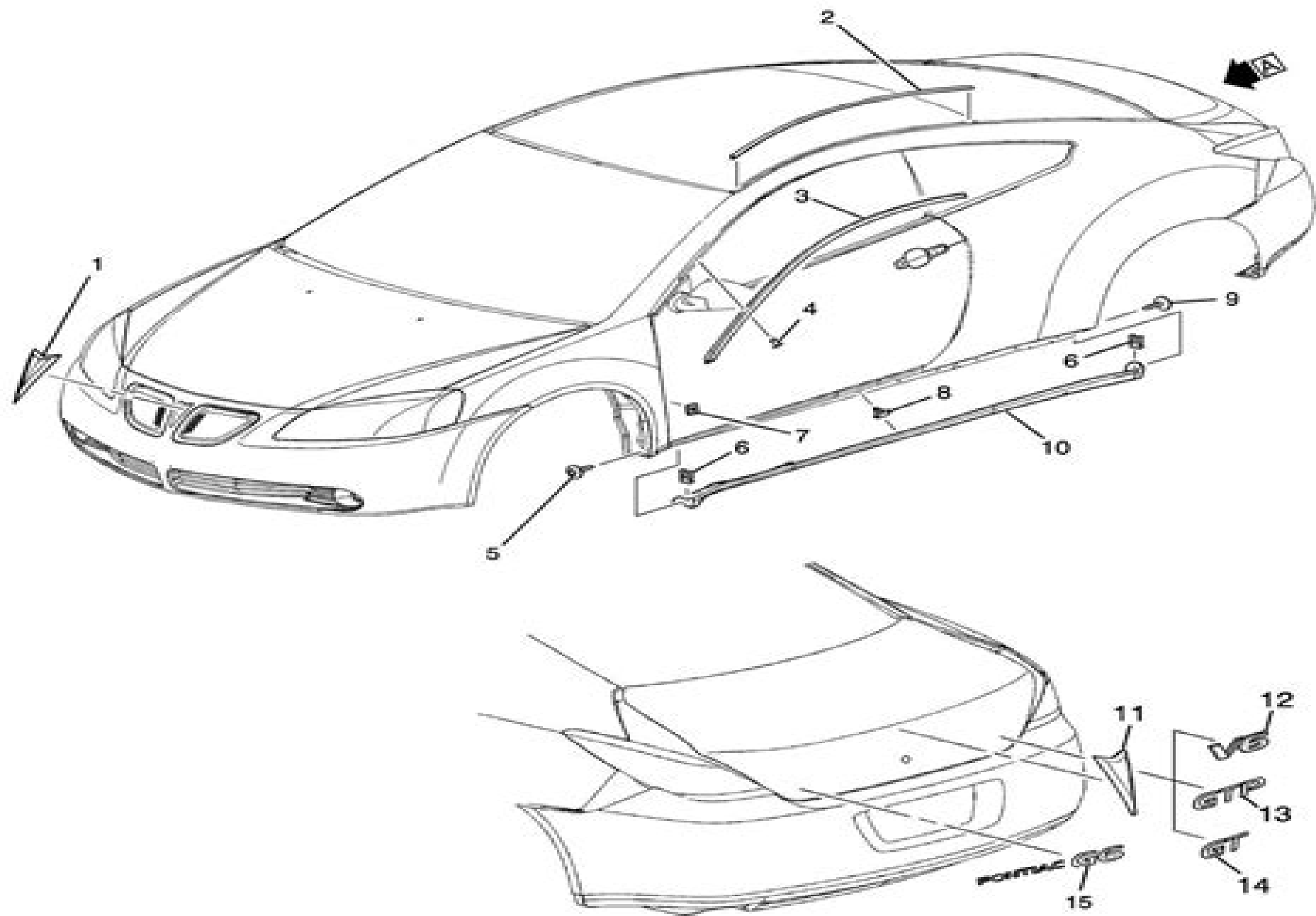
VIEW A
