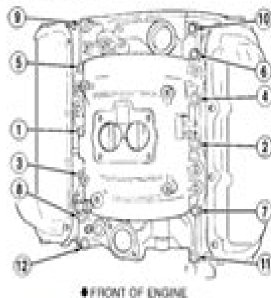
Fig. 5: Intake Manifold Bolt Tightening Sequence (3.9L) Courtesy of Chrysler Corp.
