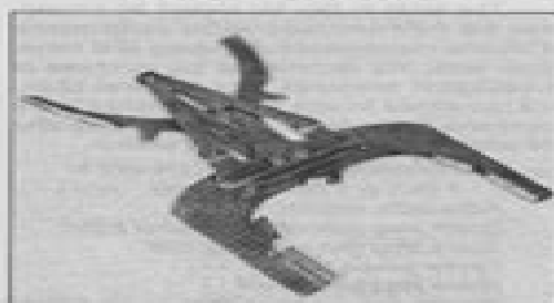
Ring removal/installation tool
