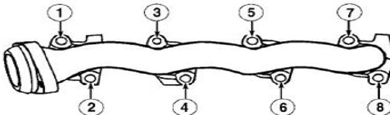
Fig. 4: Exhaust Manifold Bolt Tightening Sequence Courtesy of FORD MOTOR CO.
