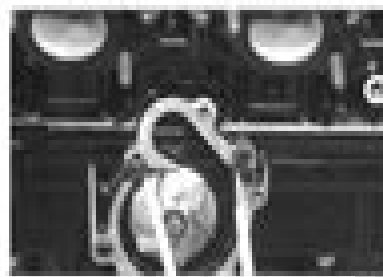
12. Position the timing into the water pump cover, then install the cover. Secure with the screws. Tighten to 1.1 kg-m (0.8 ft-lb).
