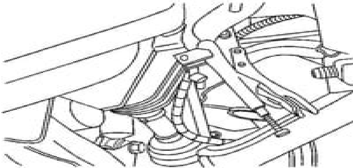
Fig. 4: Installing The Dial Indicator Between The Pitman Arm And Relay Rod Courtesy of GENERAL MOTORS CORP.
