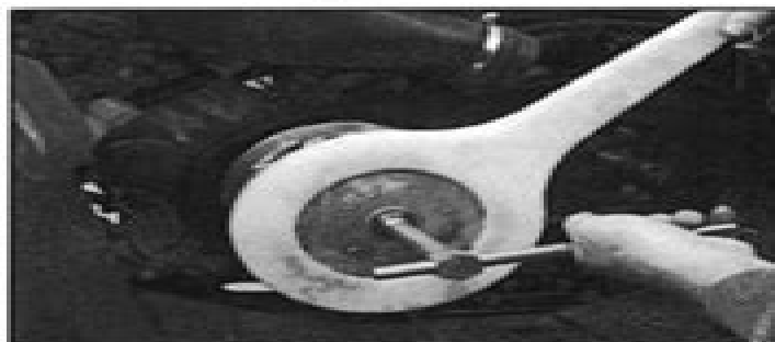
Drive Clutch Puller (PN 2870506)
