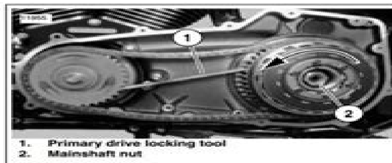
Figure 6-18. Installing Clutch Hub Mainshaft Nut
