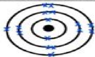
Sulfur atom
