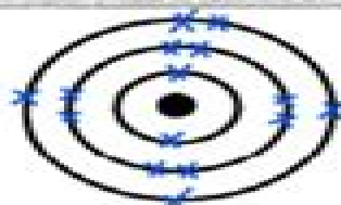
Phosphorus atom
