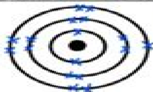
Chlorine atom
