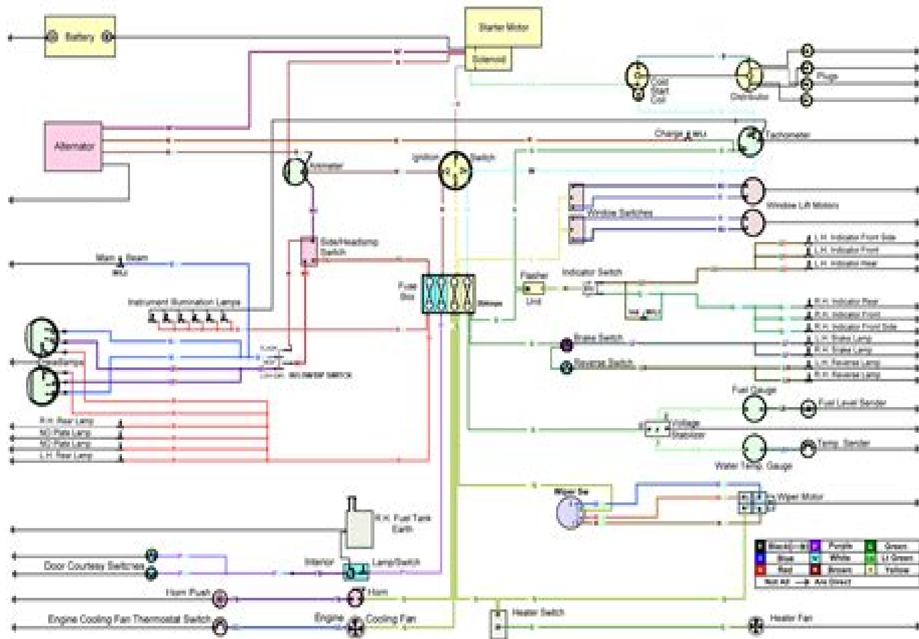
Europa Twin-Cam Wiring Diagram (U.K.)
