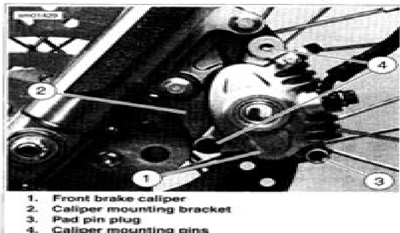
Figure 1-23. Front Caliper Assembly
