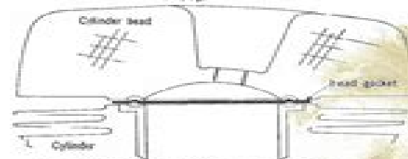
Fig. 6-1-2 Installing cylinder head gasket
