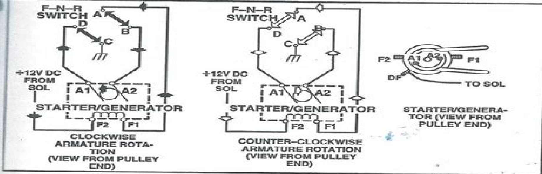
FIG. L-3 CIRCUIT DIAGRAM, STARTER/GENERATOR DIRECTION - LATER 1990
