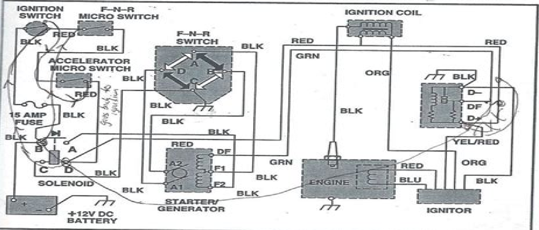
FIG. L-3 CIRCUIT DIAGRAM, STARTER/GENERATOR DIRECTION - LATER 1990
