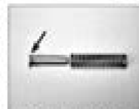
10.34 Ensure that the flat side (arrowed) of the oil pump side oil head is facing toward the top of the timing cover.
