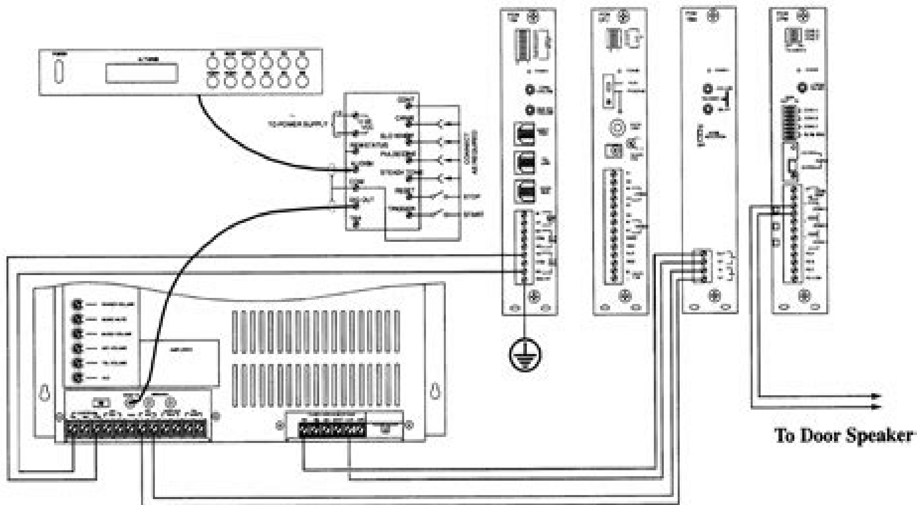
Figure A-7: Typical Connection to Operate a Door Speaker
