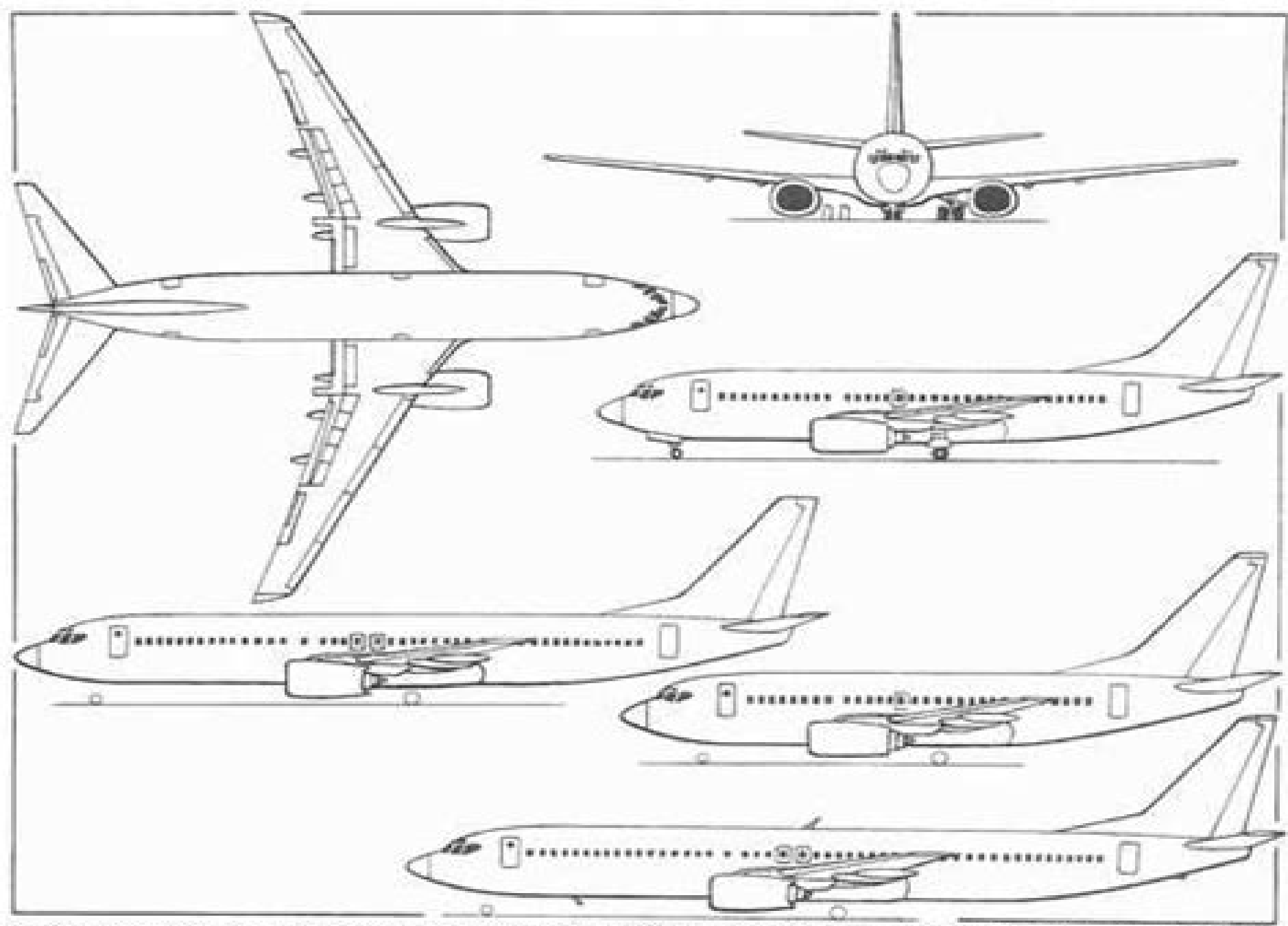
Boeing 737-700, with additional side views of stretched -800, shorter -600 and further stretched -900 (bottom) (James Goulding)
