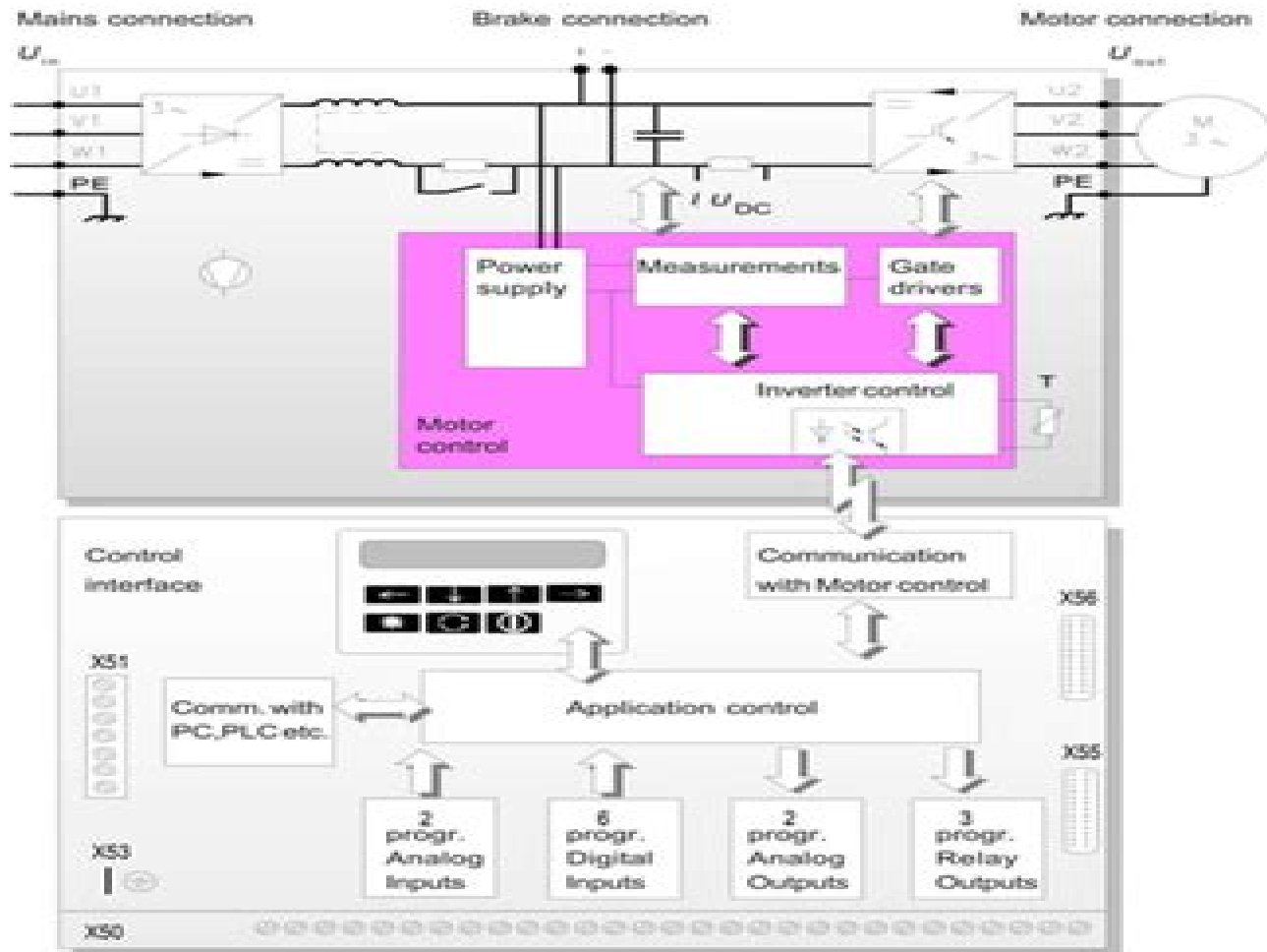
Figure 3-1. SAMI GS block scheme.
