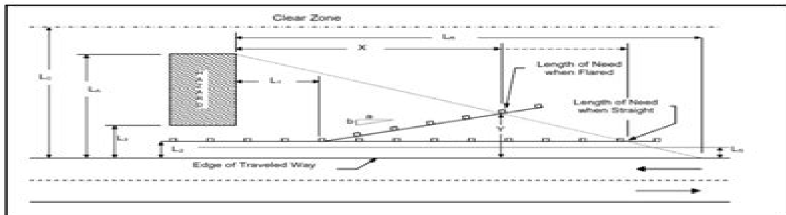
Figure 4.1: Barrier Design Variables
