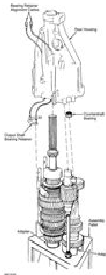
Fig. 8. Installing Rear Bearing (TWD) Courtesy of GENERAL MOTORS CORP.
