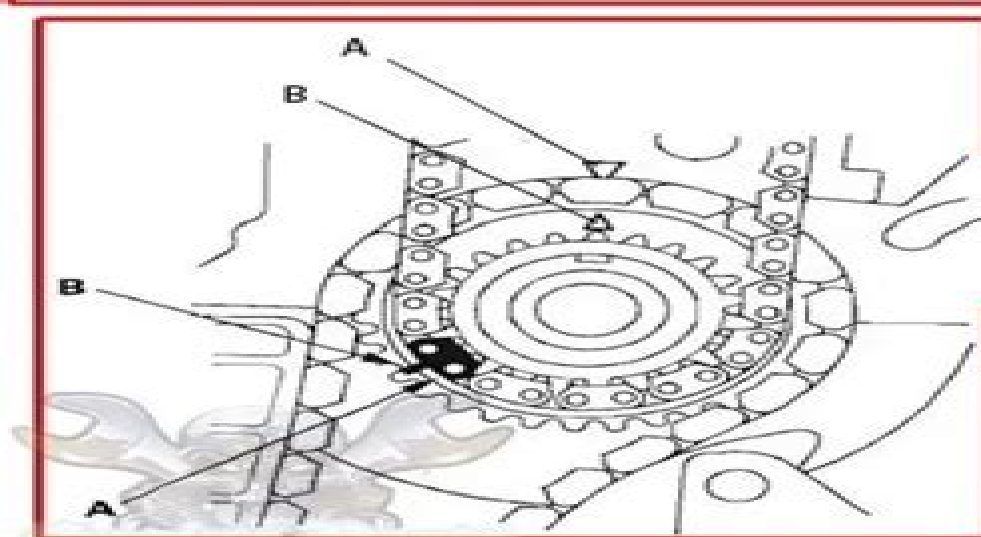
Honda K-series Engine Timing Marks Diagram
