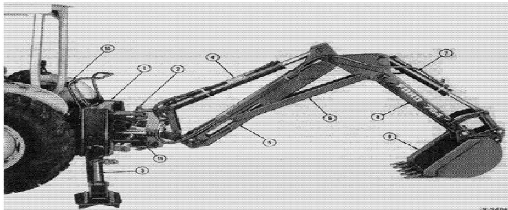
Figure 1 Backhoe Components 5. Boom 6. Long Bar Link 7. Bucket Cylinder 8. Dipperstick
