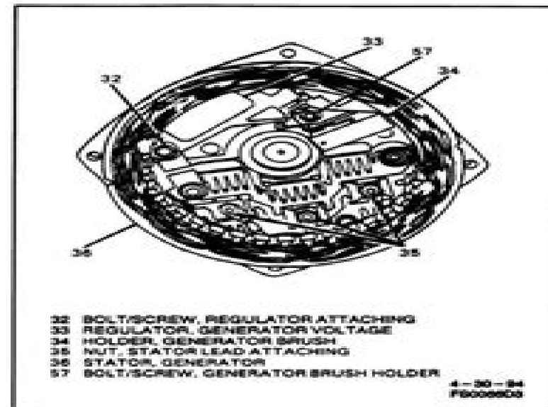
Figure 6 - Generator Slip Ring End Frame View
