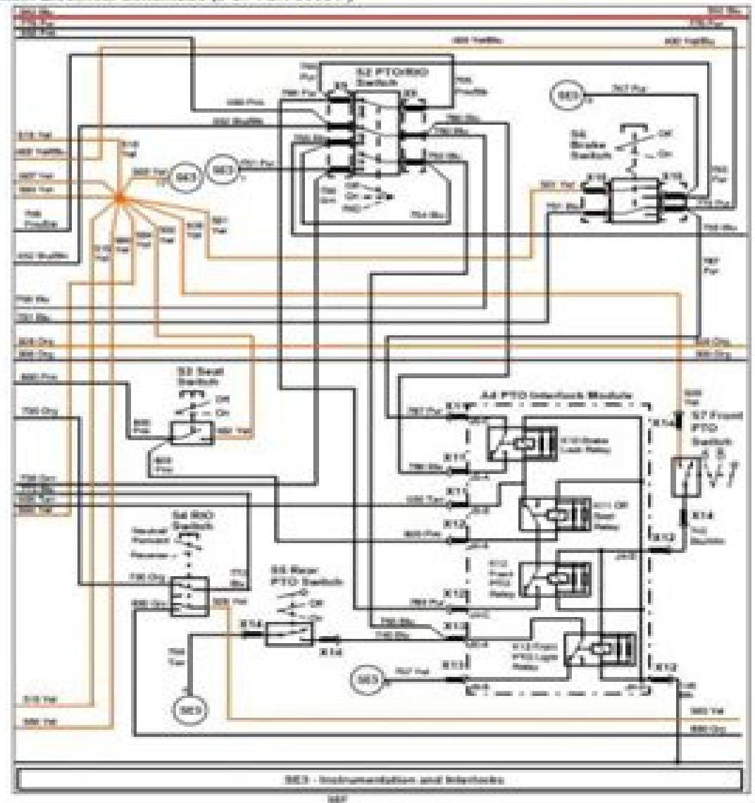
Main Electrical Schematic (3 of 4 SN 30001-)
