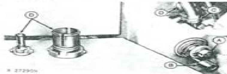
A—Engine Rotation Tool B—Timing Pin C—Crankcase Vent Hose D—Plastic Plugs
