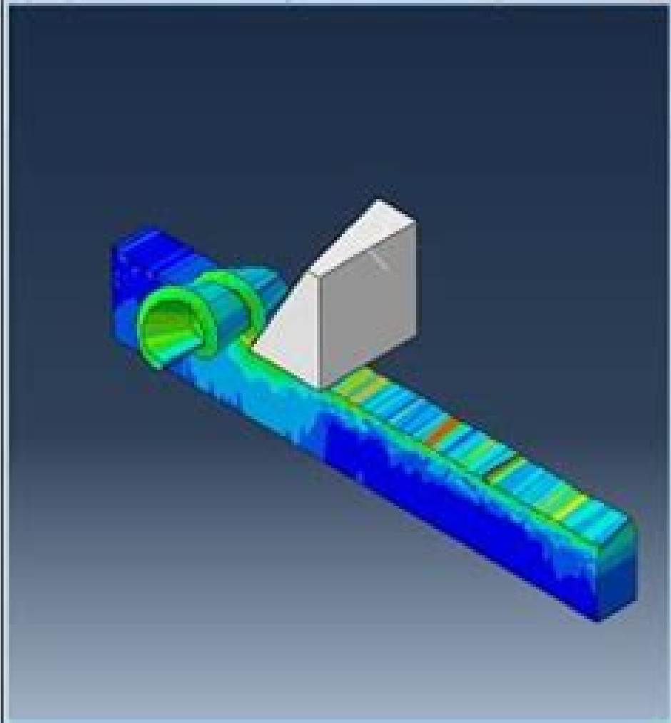
Viewport 2 009: C:\YouTube\CAE_Models\Johnson-Cook\Cutting.off
