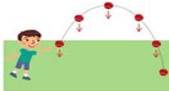
Trajectory of a ball thrown in air
