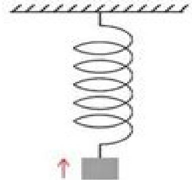
Weight on a spring
