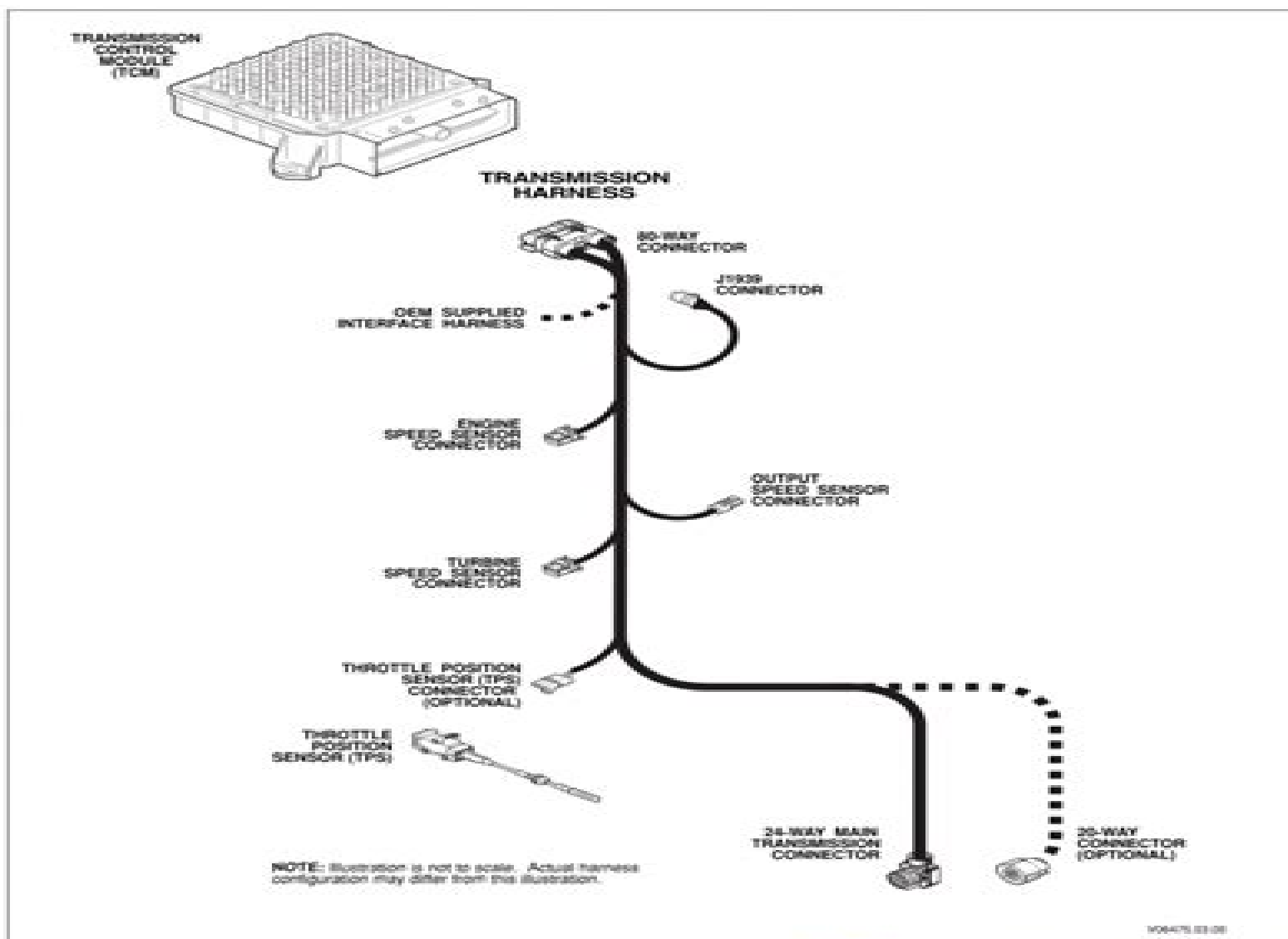
Figure 1-10. Typical External Wiring Harnesses
