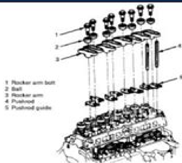
Fig. 2: 2.5L rocker arm components
