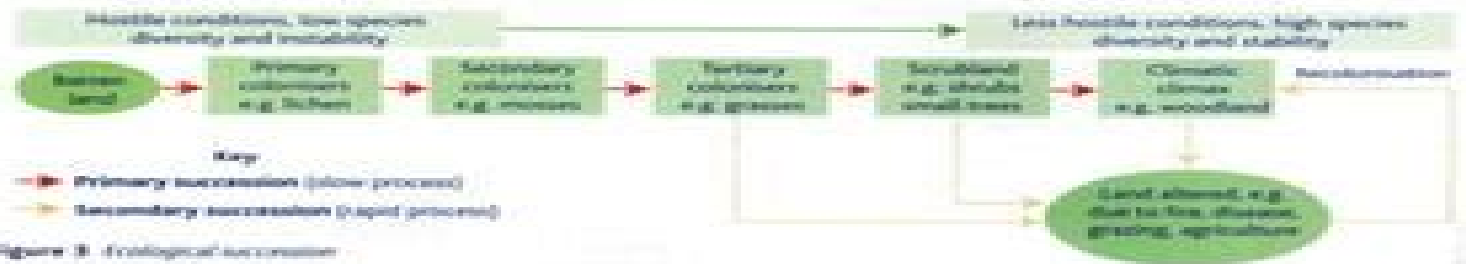
Figure 3 summarises the events of ecological succession on land.
