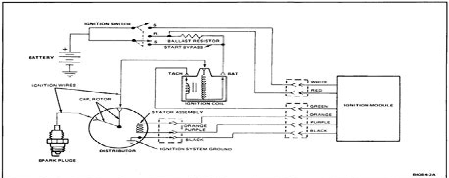
FIG. 9 Typical Duraspark II Ignition System
