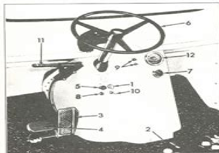
Figure 1A-6. Controls - 1969-1972 Model DC
