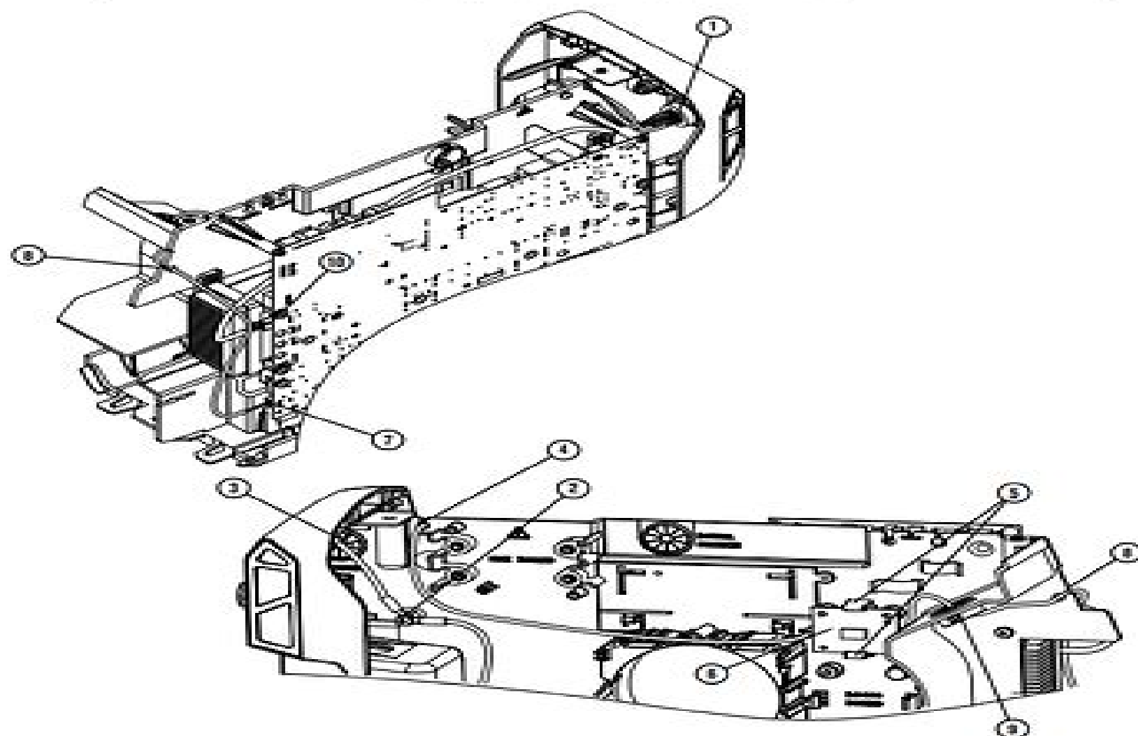
Figure 36 – Machine interface (CPC port) cable routing (internal components omitted for clarity)
