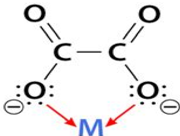
Oxalate
