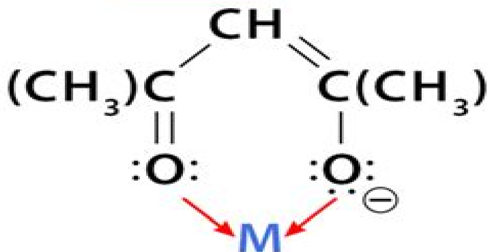
Acetylacetonate
