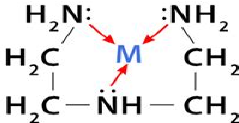
Diethylenetriamine
