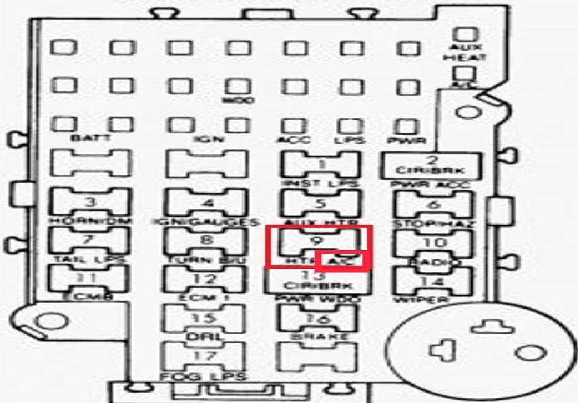
Fig. 1: Fuse Panel Identification (1990-93) Courtesy of GENERAL MOTORS CORP.
