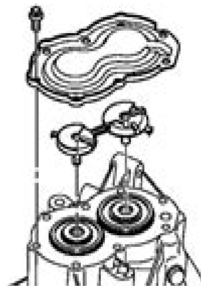
Fig. 81: View Of Rear Cover & Bolt Courtesy of GENERAL MOTORS CORP.
