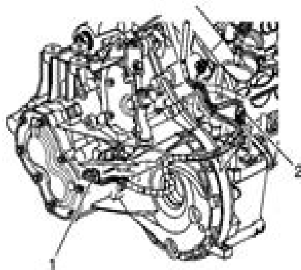
Fig. 80: Locating Backup Light Connector & YSS Connector Courtesy of GENERAL MOTORS CORP.
