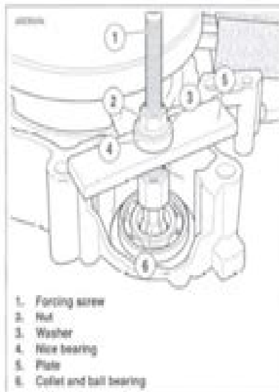
Figure 3-176. Removing Balance Support Bearings
