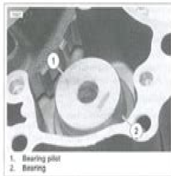
Figure 3-177. Balance Support Bearing Pilot
