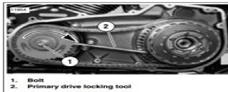
Figure 6-17. Installing Compensating Sprocket Nut
