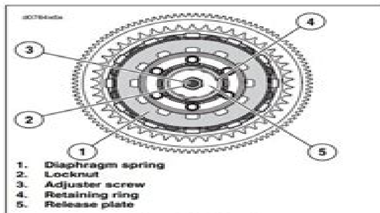
Figure 6-19. Clutch
