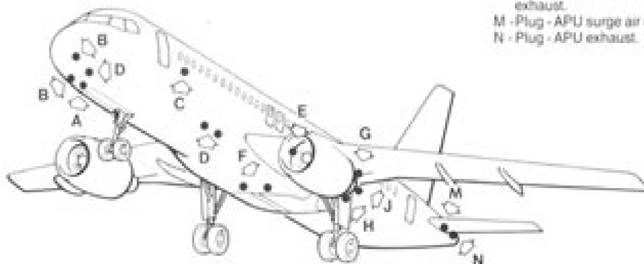
Fig. 10-1 Airframe covers-location www.british-caledonian.com
