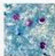
Cryptosporidium sp.
