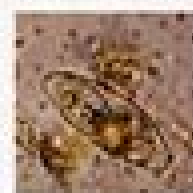
Isospora sp.
